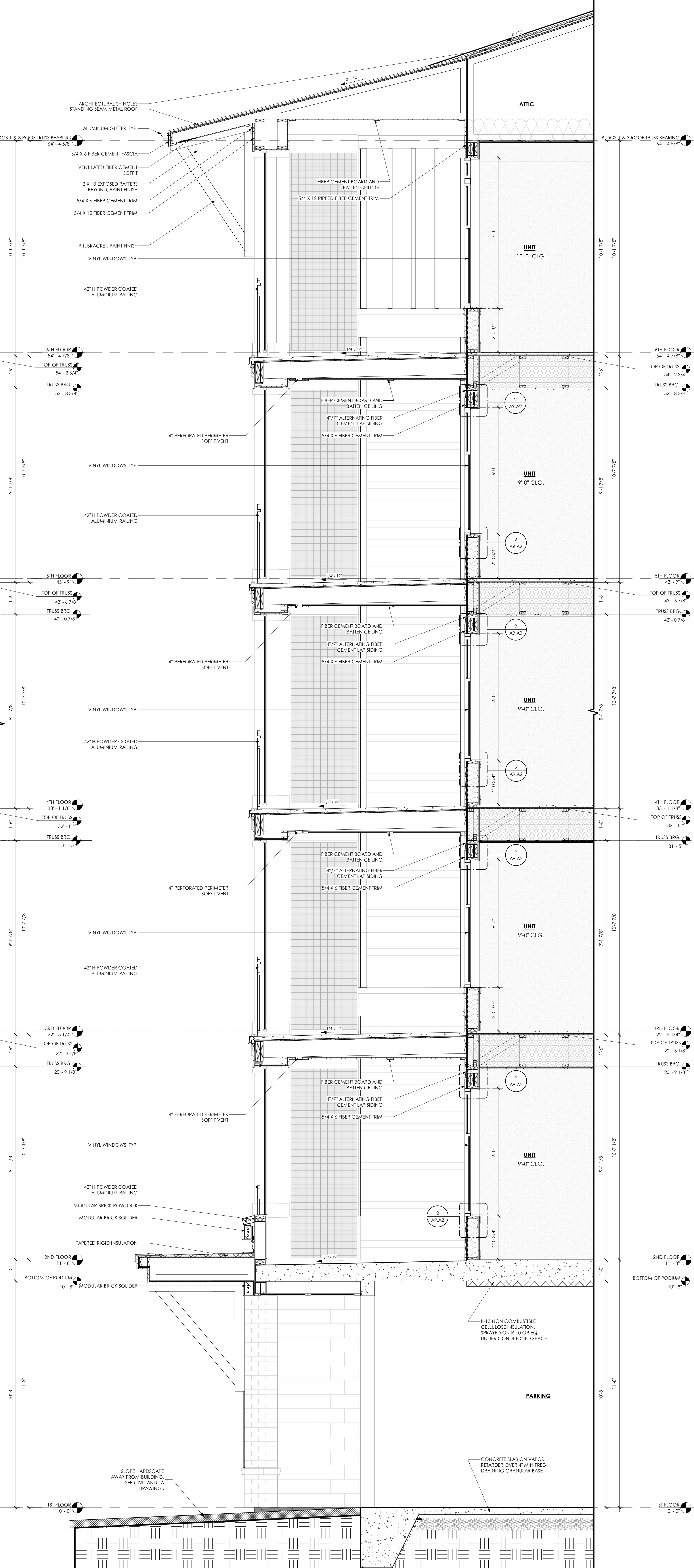
TYPICAL WALL SECTION AT A STORY LOW ROOF AT BALCONIES AT WINDOW AT GARAGE
